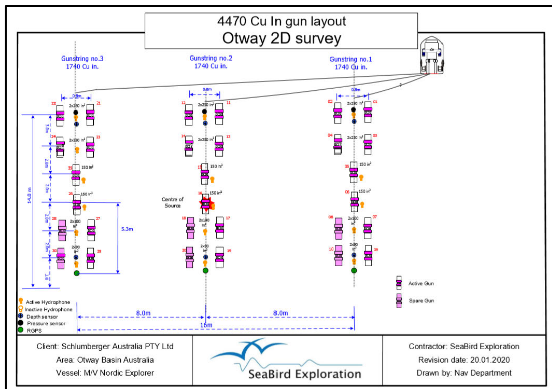
Figure 5 Gun array configuration
