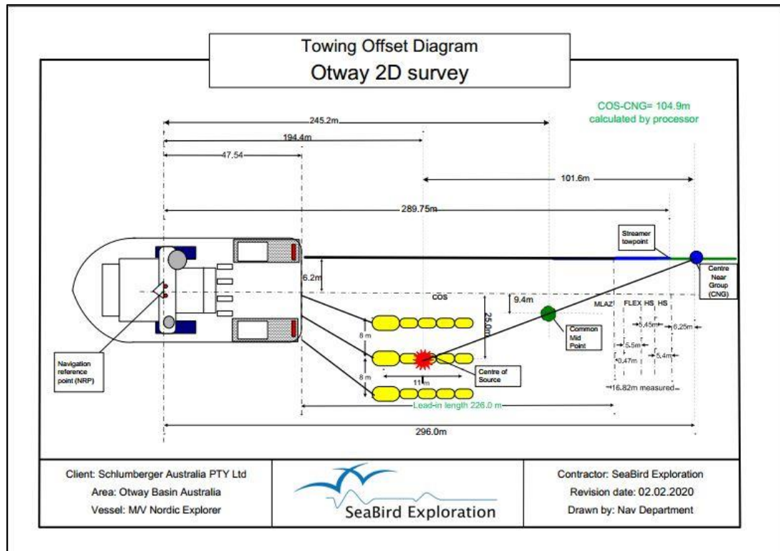
Figure 4 Source and streamer configuration and distances
